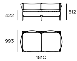
Divano 2 posti sofa, 2-Sitzer-Sofal
