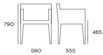
Poltroncina Monet dining armchair, armlehnstuh
