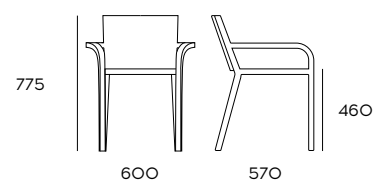
Poltroncina impilabile Van Gogh stackable dining chair, stapelbarer stuhl
